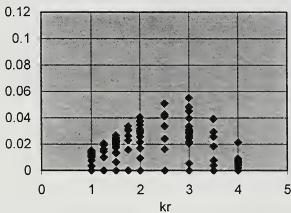
Figure 8. Normalized scattered pressure deviation computed by ATILA versus kr for monopolar and dipolar incident fields.
